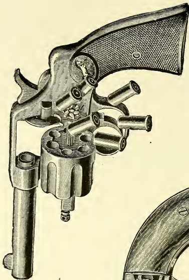
The Colt Self-ejecting Revolver.
